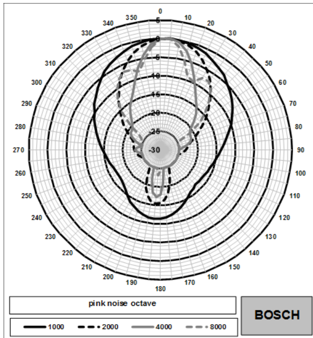
Polar diagram LH1-CC30-IN (Octave band frequency in Hz)
